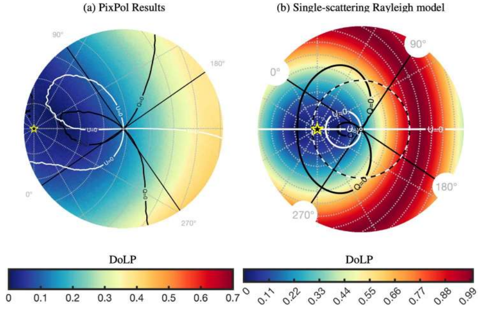
Figure 40. In-water upwelling DoLP_{\text{water}} ( \lambda = 670 \text{ nm} ). The measured Q=U=0 location occurs interior of the refracted anti-solar point near the principal plane.
