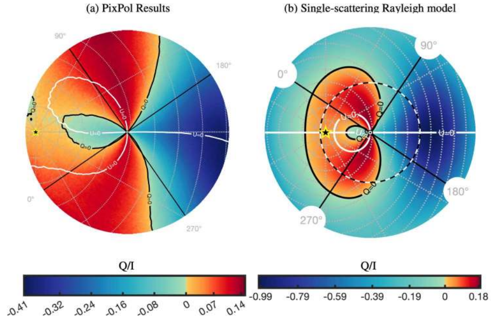
Figure 38. In-water upwelling Q_{\text{water}}/I_{\text{water}} ( \lambda = 670 nm).
