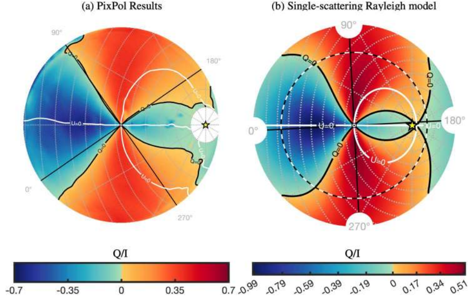
Figure 33. Downwelling Q_{\text{sky}}/I_{\text{sky}} ( \lambda = 500 nm). In the measured image, the Q=0 line on the solar half does not close the interior of the solar direction and indicates a contribution of light linearly polarized perpendicular to the principal plane.
