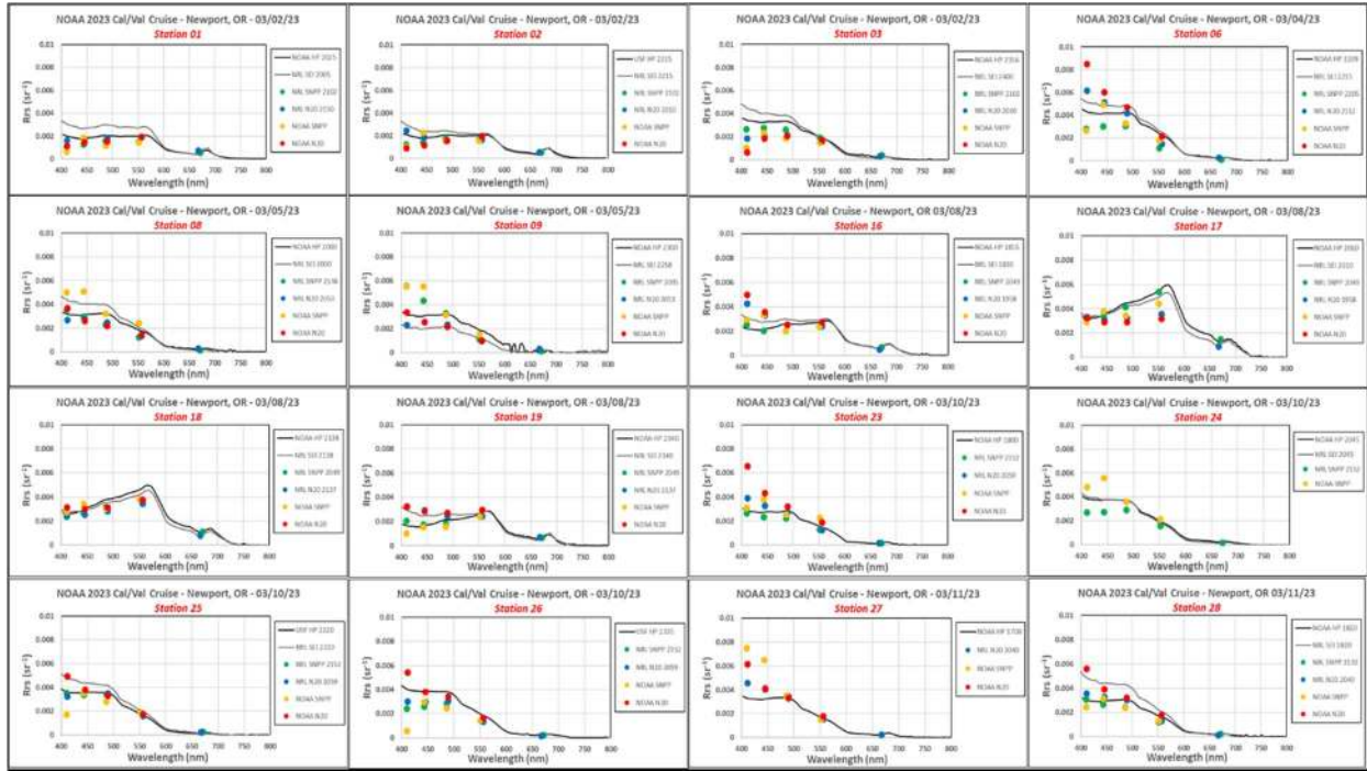
Figure 44. Comparison of the R_{rs} spectra measured in situ and satellites during the Cal/Val cruise.
