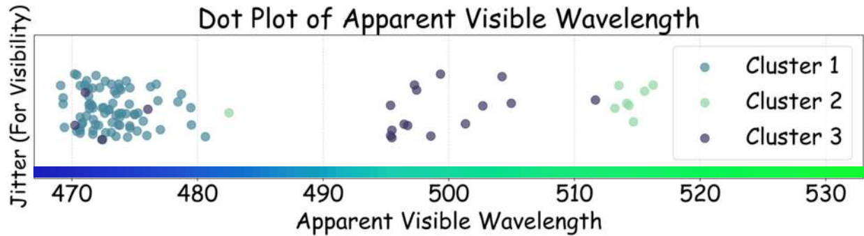
Figure 29. Apparent visible wavelengths of spectra colored by their cluster group. The apparent visible wavelength is a relatively good metric for determining water type as this highly reductive method (going from hundreds of points in a hyperspectral dataset down to one representative wavelength) aligns with the results of the clustering algorithm quite well, with a few exceptions.
