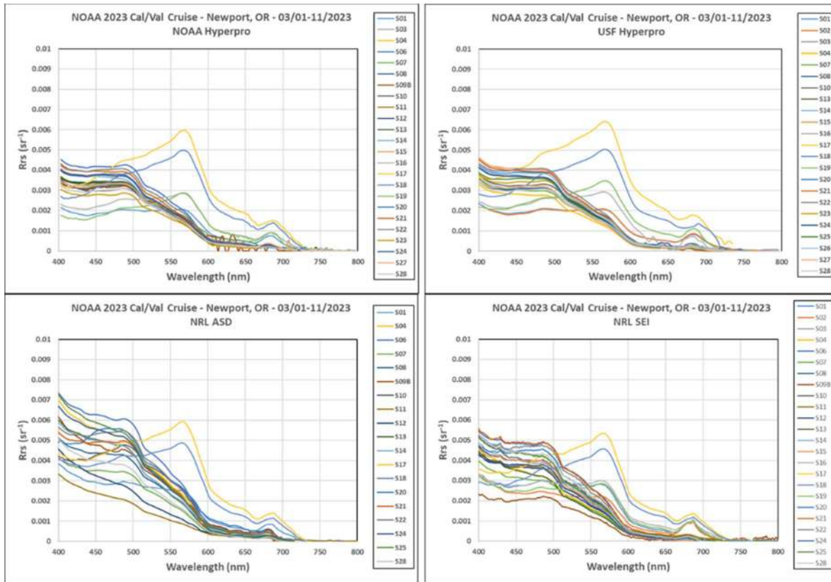
Figure 42. R_{rs} spectra collected by the NOAA (top left) and USF (top right) profiling HyperPro's and NRL's above-water ASD (bottom left) and SEI (bottom right) radiometers. Legends are given for the station numbers.
