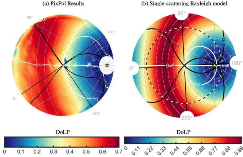
Figure 35. Downwelling DoLP_{sky} ( \lambda = 500 nm). The maximum DoLP occurs near a 90^\circ scattering angle as predicted by the single-scattering Rayleigh model. However, unlike the model, the measured the Q=U=0 location does not occur along the principal plane.
