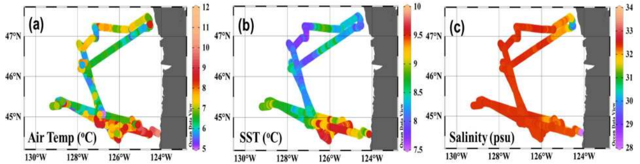
Figure 16. Distribution of a) Air temp b) SST, c) Salinity.
