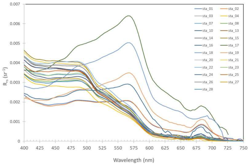
Figure 23. R_{rs}(\lambda) estimated from HyperPro-II profiles at SH23-02 stations.
