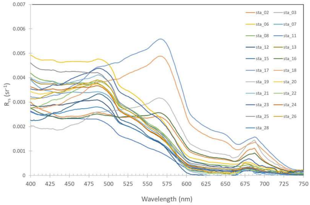
Figure 22. R_{rs}(\lambda) derived from above-water SVC HR-512i measurements during SH23-02.
