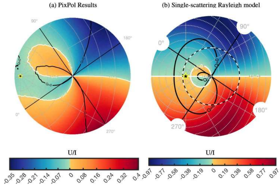
Figure 39. In-water upwelling U_{\text{water}}/I_{\text{water}} ( \lambda = 670 nm).
