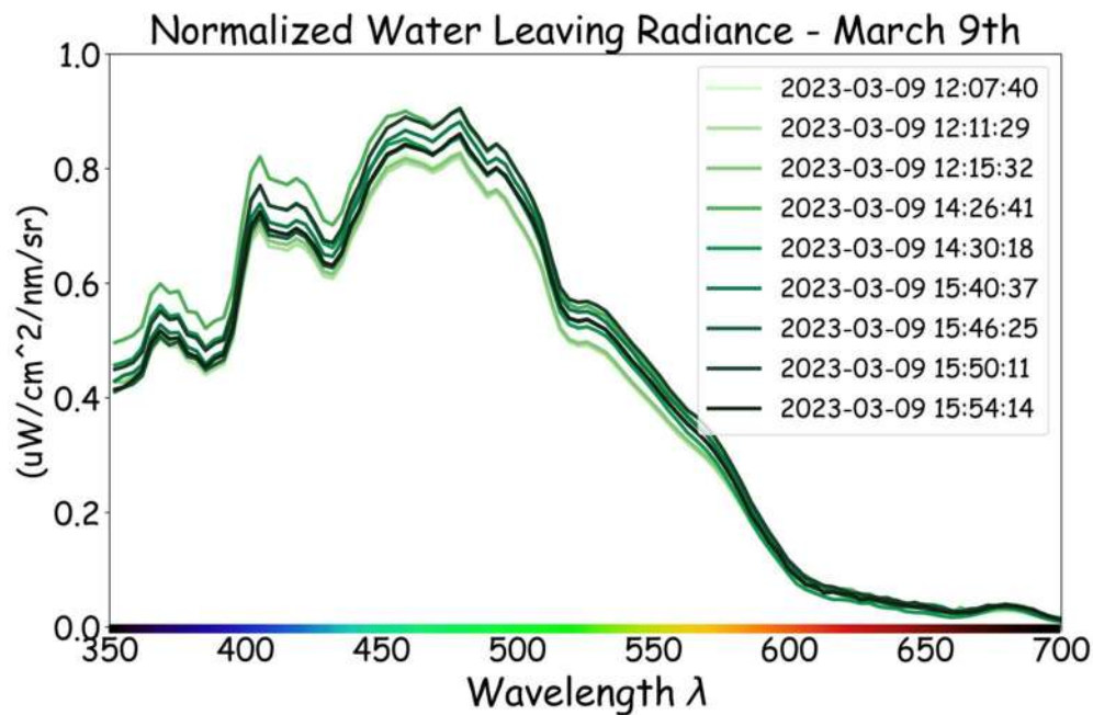
Figure 26. Example of water leaving radiance derived from OSU HyperPro-II for the 9 th of March 2023.
