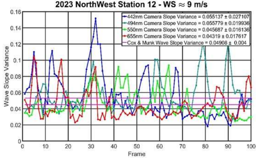
Figure 14. Estimation of wave slope variances using polarimetric sensing at Station 12.
