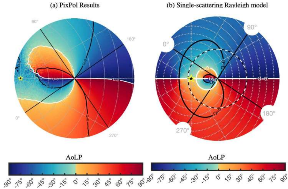
Figure 41. In-water upwelling AoLP_{\text{water}} ( \lambda = 670 \text{ nm} ).
