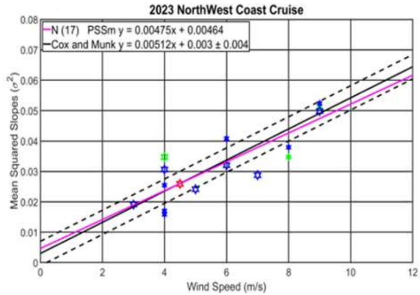
Figure 15. The camera recorded mean square slopes vs. wind speed for the 2023 cruise. The colors represent which color filter 442 nm (blue), 494 nm (cyan), 550 nm (green), or 655 nm (red) was selected. The corresponding sun zenith angle is shown by filled markers (around noon time) zenith with the angle at 25 to 35° and empty markers (morning and evening) with angles greater than 35°.
