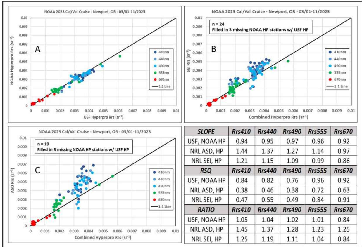
Figure 43. Scatterplots of in situ determination of R_{rs} during the Cal/Val cruise. The table (bottom right) gives the statistics (slope, r^2 , and ratio) for each comparison. “HP” and “RSQ” in the table refer to HyperPro and r^2 , respectively.
