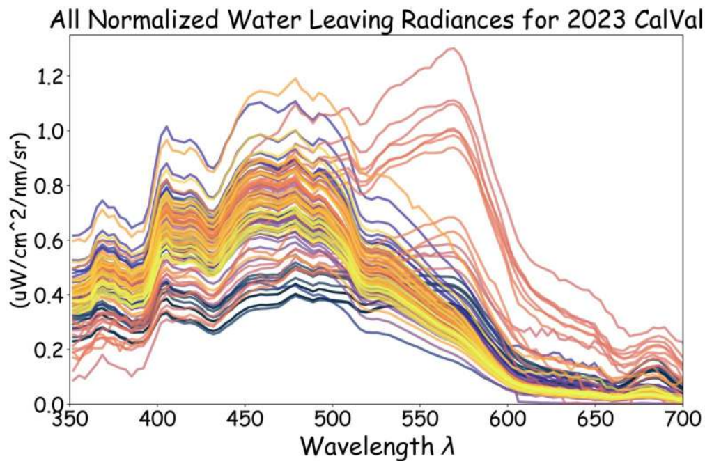
Figure 27. All water leaving radiance derived from the OSU HyperPro-II throughout the entirety of the cruise.
