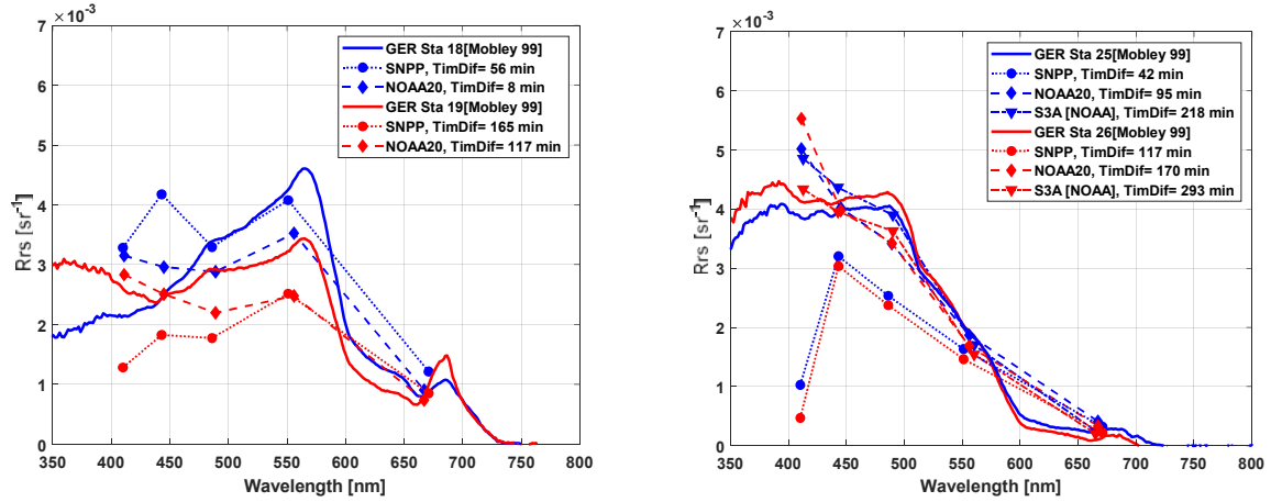
Figure 12. Comparison of measured spectra by GER and satellite data for several stations.
