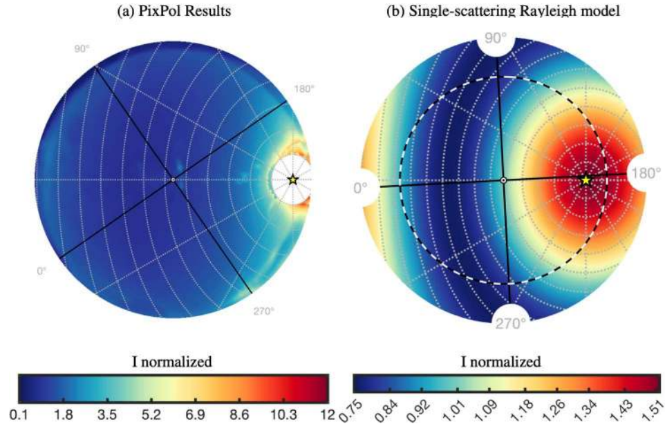
Figure 32. Downwelling I_{sky} ( \lambda = 500\text{nm} ). Values are normalized to the mean value within 2^\circ of the zenith direction. Application of this image is locating the solar position and monitoring cloud conditions.
