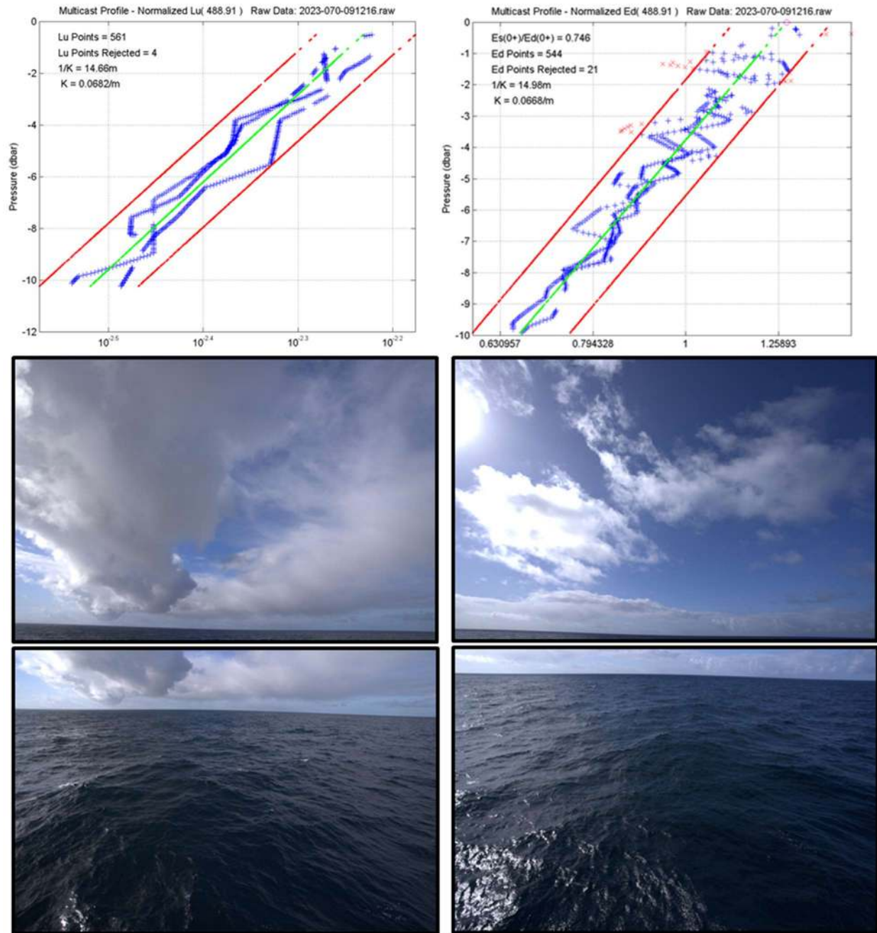
Figure 25. Examples of L_u and E_d profiles from the HyperPro-II for 488 nm and RGB pictures of the water in which the HyperPro's were deployed.
