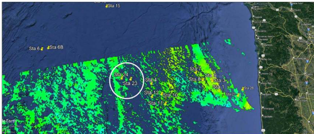
Figure 6. Satellite Chl-a image from March 10, 2023, when stations 23, 24, 25, and 26 were sampled.
