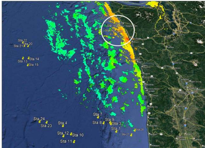
Figure 5. Satellite Chl-a image (March 8, 2023) showing stations 16, 17, 18, and 19.
