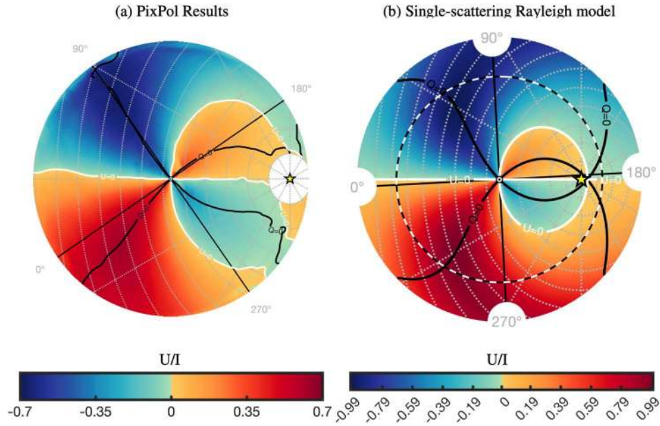
Figure 34. U_{\text{sky}}/I_{\text{sky}} ( \lambda = 500 nm).
