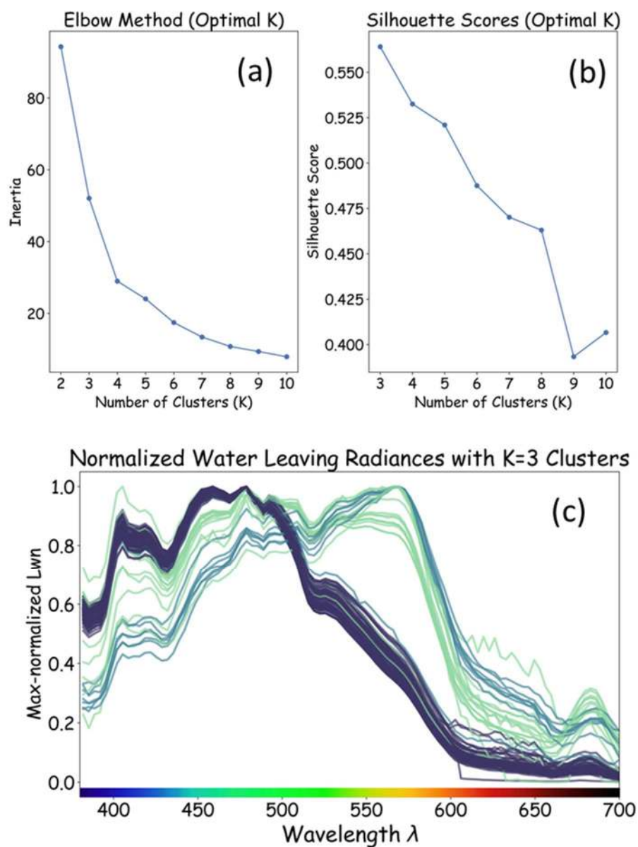
Figure 28. Elbow plot and Silhouette score for all normalized water leaving radiances (max-normalized so all individual spectra are scaled between 0 and 1) for OSU's in-water profilers. Clustered, normalized spectra are seen below with unique colors to represent each cluster. More "pure" oceanic water (dark blue) transitions into a more phytoplankton-detritus-dominated regime (light green) as we get closer to the coast.
