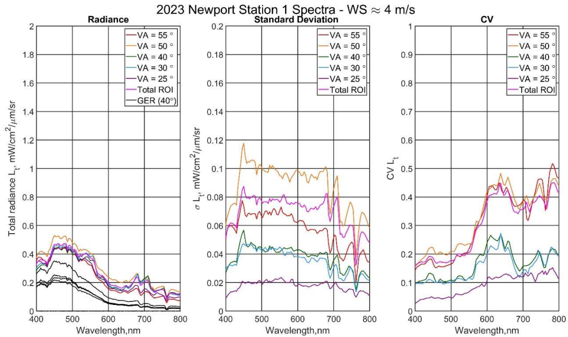
Figure 13. Data from the hyperspectral imager: above-water spectral radiances at viewing angles 25°–55° compared with GER spectra (left), radiances uncertainties (center), coefficient of variation or CV (right).
