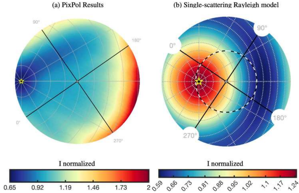
Figure 37. In-water upwelling I_{\text{water}}(\lambda = 670 \text{ nm}) . In the measured image, low radiance values are measured in the vicinity of the refracted anti-solar location where the instrument self-shading occurs. Values are normalized to the mean value within 2^\circ of the nadir direction.
