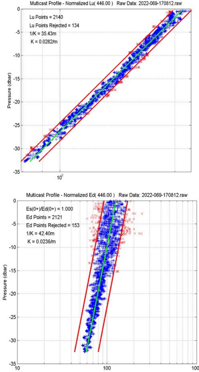
Figure 25. Examples of L_u and E_d profiles from the HyperPro-II for blue light (446 nm)
